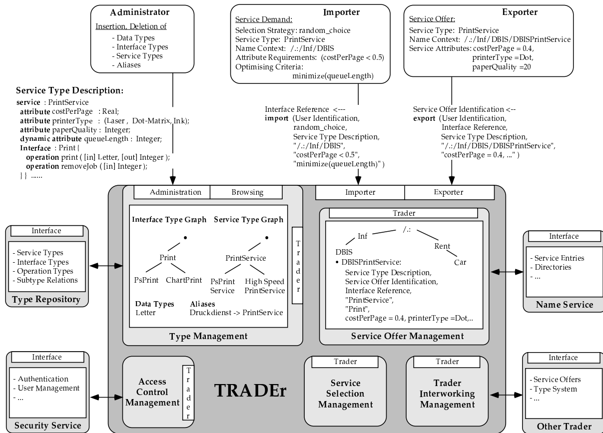
Figure 3: TRADER Components and Implementation Architecture
