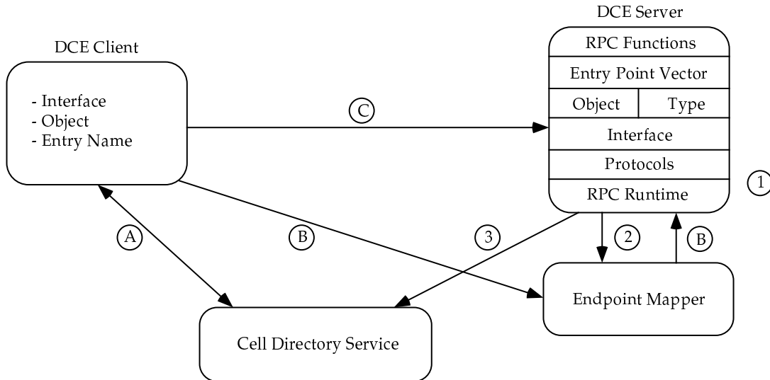
Figure 2: CDS Based Binding
