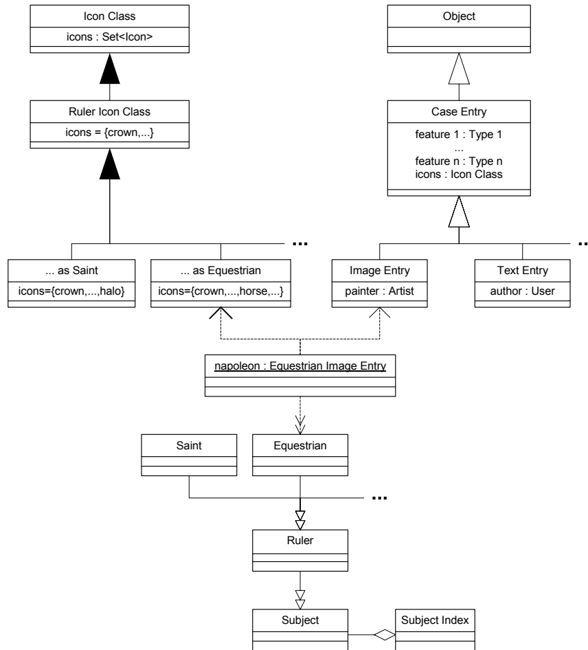
Fig. 10. Subject, object and icon classes
