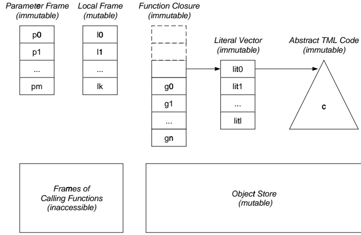
Figure 5: The TML machine model
