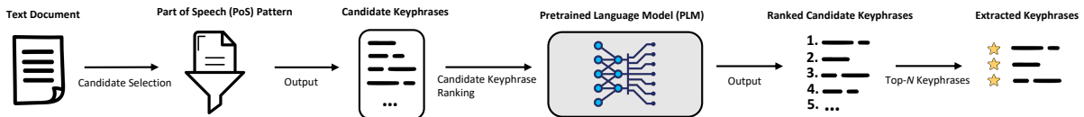
Figure 1: PatternRank approach for unsupervised keyphrase extraction. A single text document is used as input for an initial filtering step where candidate keyphrases are selected which match a defined PoS pattern. Subsequently, the candidate keyphrases are ranked by a PLM based on their semantic similarity to the input text document. Finally, the top- N keyphrases are extracted as a concise reflection of the input text document.
